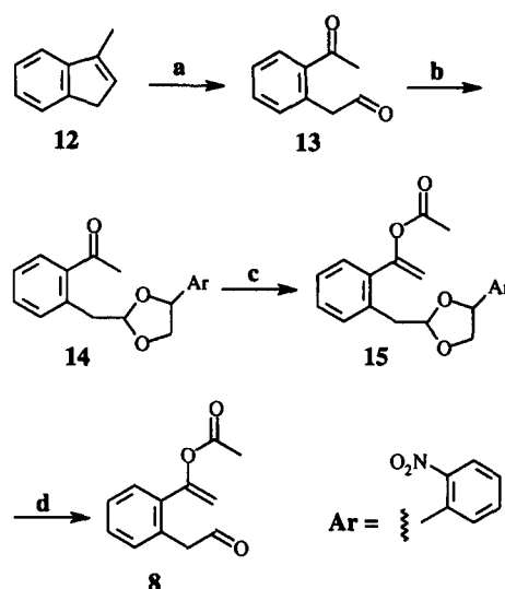
Figure 2. Reagents and conditions: (a) \text{O}_3 , \text{CH}_2\text{Cl}_2 , -78^\circ\text{C} ; \text{Zn} , \text{HOAc} , 0^\circ\text{C} (89%); (b) ortho -nitrophenylethylene glycol, para - \text{MeC}_6\text{H}_4\text{SO}_3\text{H} , benzene, reflux (52%); (c) \text{KHMDS} , \text{DME} , -78^\circ\text{C} ; \text{CH}_3\text{C}(\text{O})\text{Cl} , \text{DMAP} , -78^\circ\text{C} (52%); (d) h\nu (350 nm), benzene, rt (45%).
