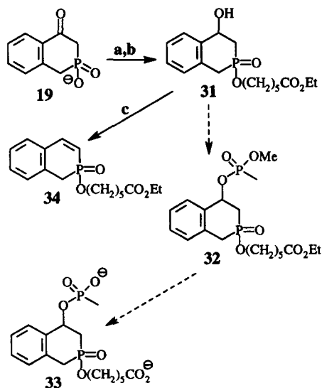
Figure 5. Reagents and conditions: (a) Br(CH 2 ) 5 CO 2 Et, KI, K 2 CO 3 , DMF ~70 °C, (30%); (b) NaBH 4 , CeCl 3 ·6H 2 O, CH 3 OH, rt (80%); (c) CH 3 P(O)Cl 2 , i Pr 2 NEt, 1H-tetrazole, THF, 0 °C to rt; CH 3 OH.
