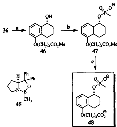
Figure 8. Reagents and conditions: (a) 45 , \text{BH}_3\cdot\text{Me}_2\text{S} , THF, approximately −15 °C (93%); (b) \text{CH}_3\text{P}(\text{O})\text{Cl}_2 , i\text{Pr}_2\text{NEt} , 1H-tetrazole, THF, 0 °C to rt; \text{H}_2\text{O} (62%); (c) 0.25 N LiOH, \text{CH}_3\text{CN} , rt (~100%).
