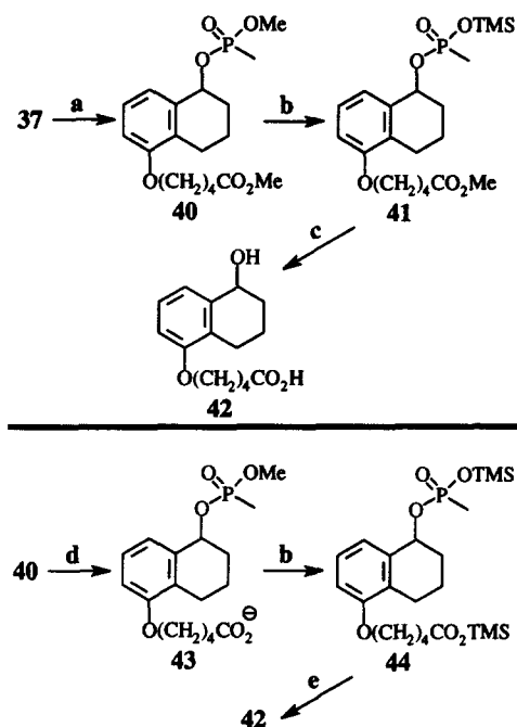
Figure 7. Reagents and conditions: (a) \text{CH}_3\text{P}(\text{O})\text{Cl}_2 , i\text{Pr}_2\text{NEt} , 1H-tetrazole, THF, 0 °C to rt; \text{CH}_3\text{OH} (75%); (b) \text{Me}_3\text{SiBr} , \text{CH}_2\text{Cl}_2 , rt; (c) 0.5 N NaOH, \text{CH}_3\text{CN} ; (d) 0.25 N LiOH, \text{tert-BuNH}_2 , rt (68%); (e) dilute aq HCl.
