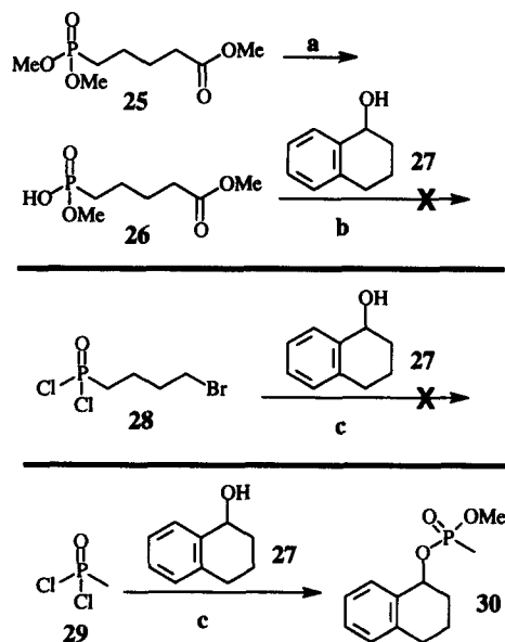
Figure 4. Reagents and conditions: (a) tert - \text{BuNH}_2 , rt (~100%); (b) 27 , i\text{PrO}_2\text{CN}=\text{NCO}_2i\text{Pr} , \text{PPh}_3 , THF, rt; (c) 27 , \text{Et}_3\text{N} , 1H-tetrazole, benzene, 0\text{ }^\circ\text{C} to rt; \text{CH}_3\text{OH} ; (d) 27 , i\text{Pr}_2\text{NEt} , 1H-tetrazole, benzene, 0\text{ }^\circ\text{C} to rt; \text{CH}_3\text{OH} (48%).
