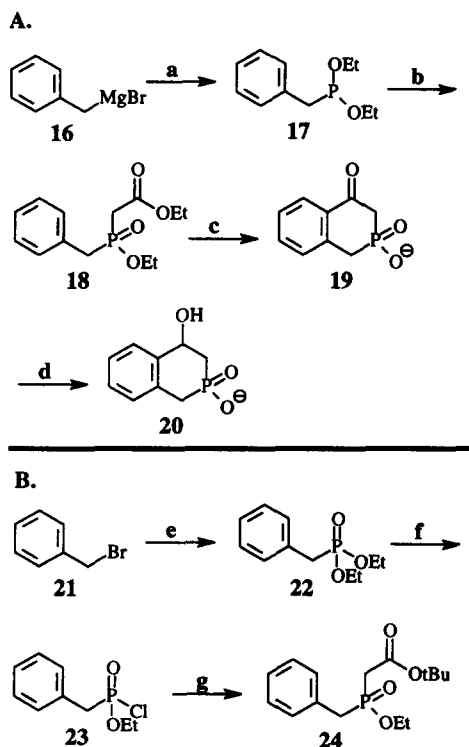
Figure 3. Reagents and conditions: (a) \text{P}(\text{OEt})_3 , \text{Et}_2\text{O} /benzene, rt; (b) \text{ClCH}_2\text{CO}_2\text{Et} , neat (17% from 16 ); (c) (i) concd \text{HCl} , reflux; (ii) polyphosphoric acid, 130\text{ }^\circ\text{C} ; \text{H}_2\text{O} (17%); (d) \text{NaBH}_4 , \text{CeCl}_3 \cdot 6\text{H}_2\text{O} , \text{CH}_3\text{OH} , rt (87%); (e) \text{P}(\text{OEt})_3 , xylene, reflux (80%); (f) \text{PCl}_5 , benzene, reflux; (g) \text{CH}_3\text{CO}_2\text{tBu} , LDA, THF, -78\text{ }^\circ\text{C} ; 23 , -78\text{ }^\circ\text{C} (31% from 22 ).
